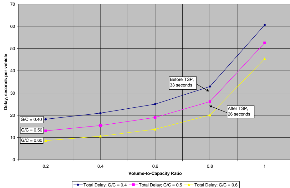
EXHIBIT 4-45 Effect of TSP on Signalized Intersection Delay (90-Second Cycle)
