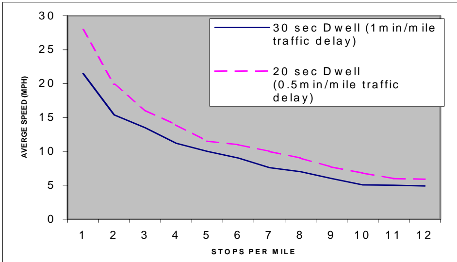
SOURCE: TCRP Research Results Digest 38 (26) EXHIBIT 4-121 Relationship Between Arterial Street Bus Speeds, Stop Frequency, and Dwell Times
