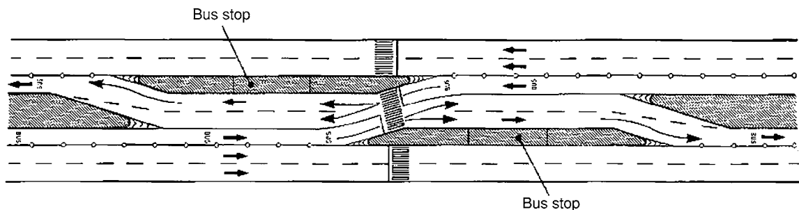
Figure 3. Typical median busway design, South America.
