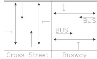
Figure 6-2. Two-phase signal phasing for separated right-of-way busway intersections.
