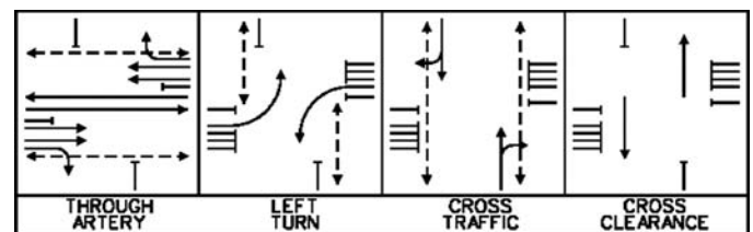
Figure 6-3. Example signal timing for median busway intersection.
