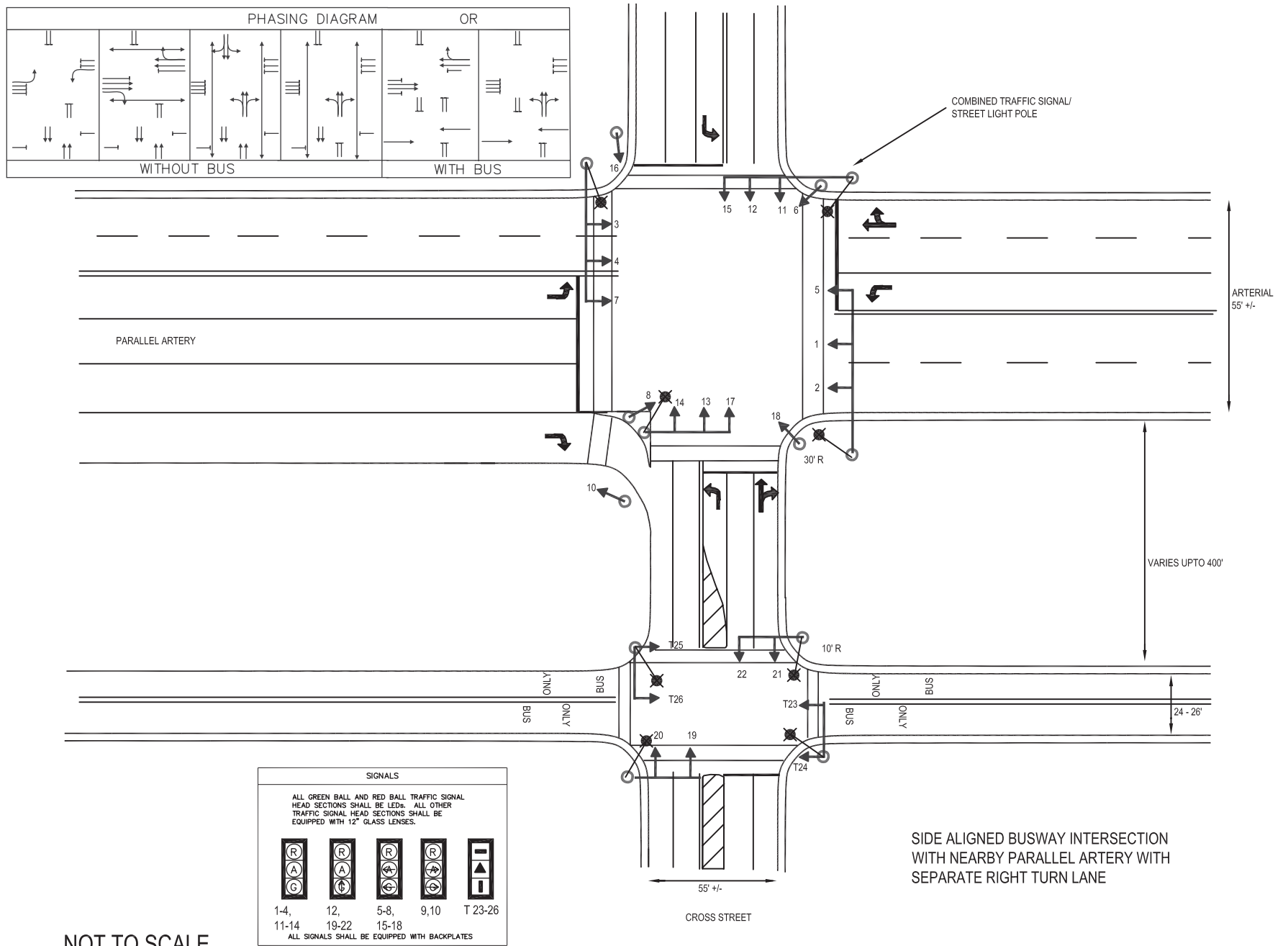
Figure 7-2. Example of a side-aligned busway intersection.
