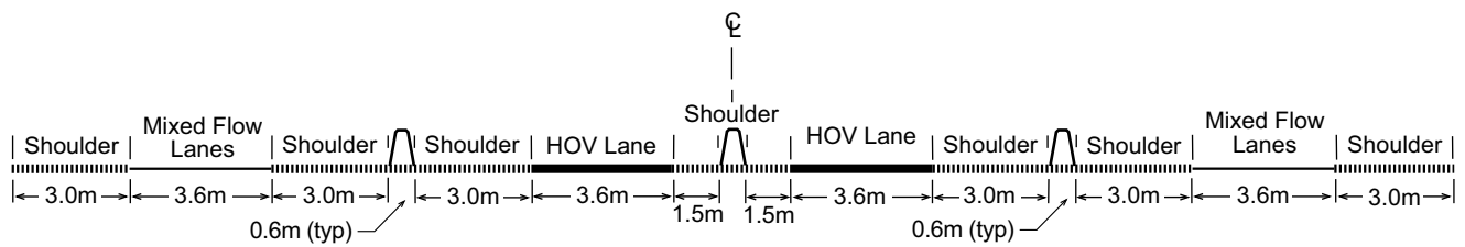
TWO-WAY BARRIER-SEPARATED HOV FACILITY
