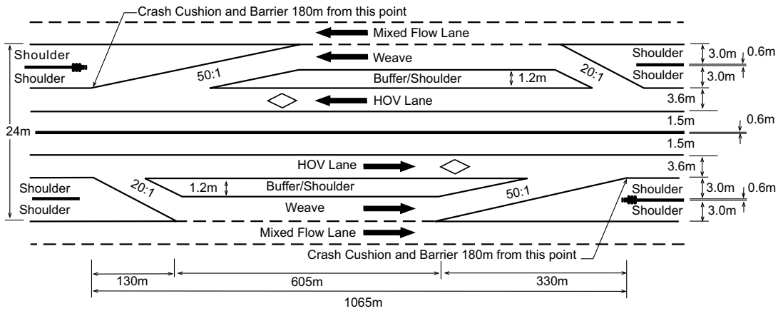
FOR 1.2m BUFFER/SHOULDER AREA
