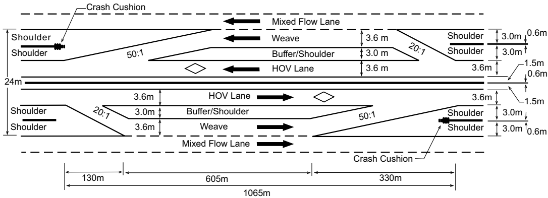
FOR 3.0m BUFFER/SHOULDER AREA
