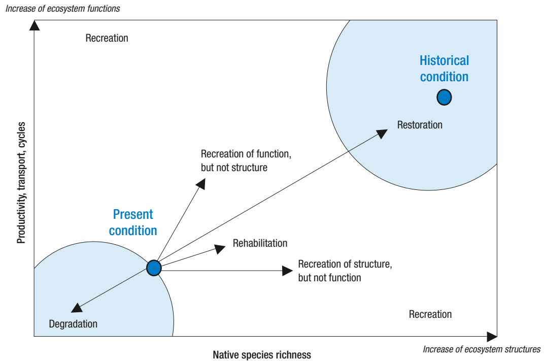
Figure 3.1: The role of ecological structures and functions in rehabilitation (Williams et al. 1997). The recreation of natural processes causes an increase of ecosystem structures (species richness, complexity of the biocoenosis) and ecosystem functions.
