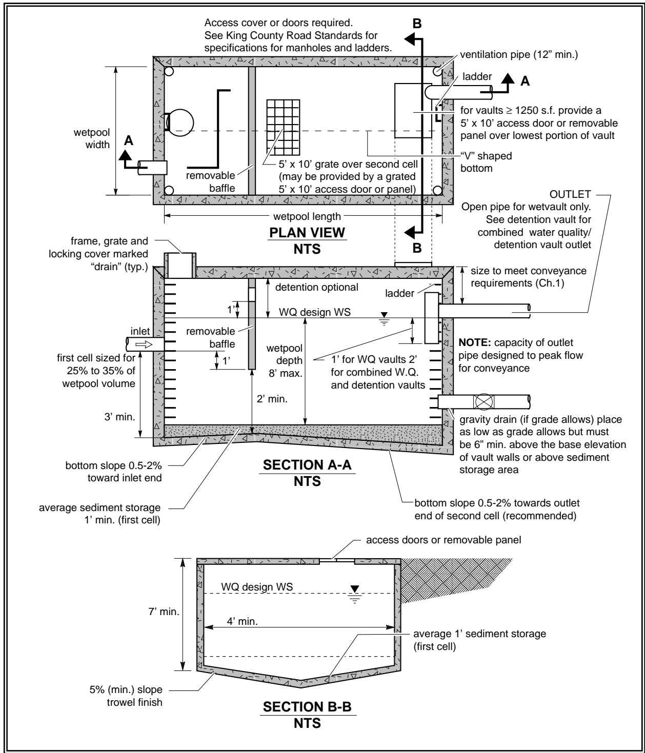
Figure 10.6 – Wetvault
