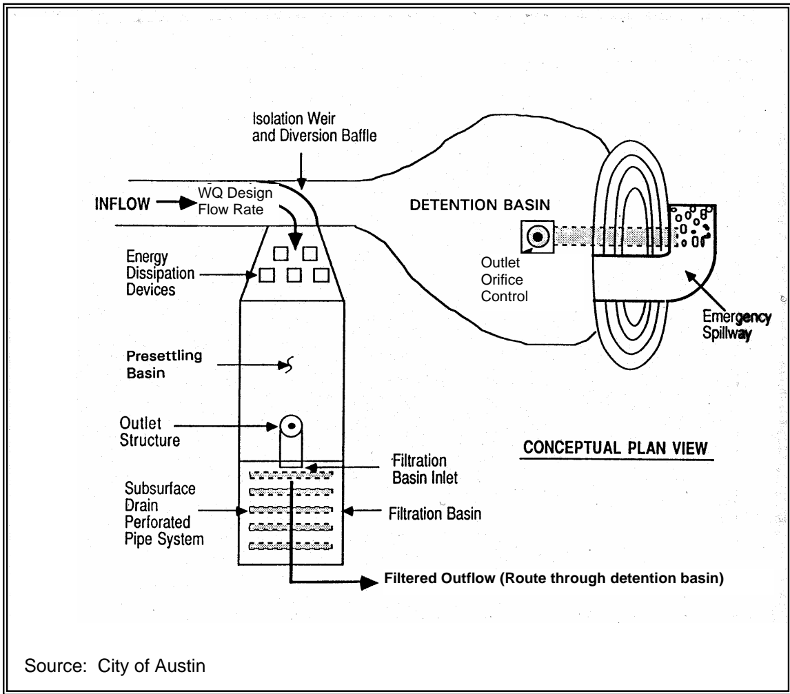
Figure 8.1 – Sand Filtration Basin Preceded by Presettling Basin (Variation of a Basic Sand Filter)
