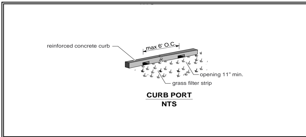
Figure 4.6 Flow Spreader Option D: Through-Curb Port
