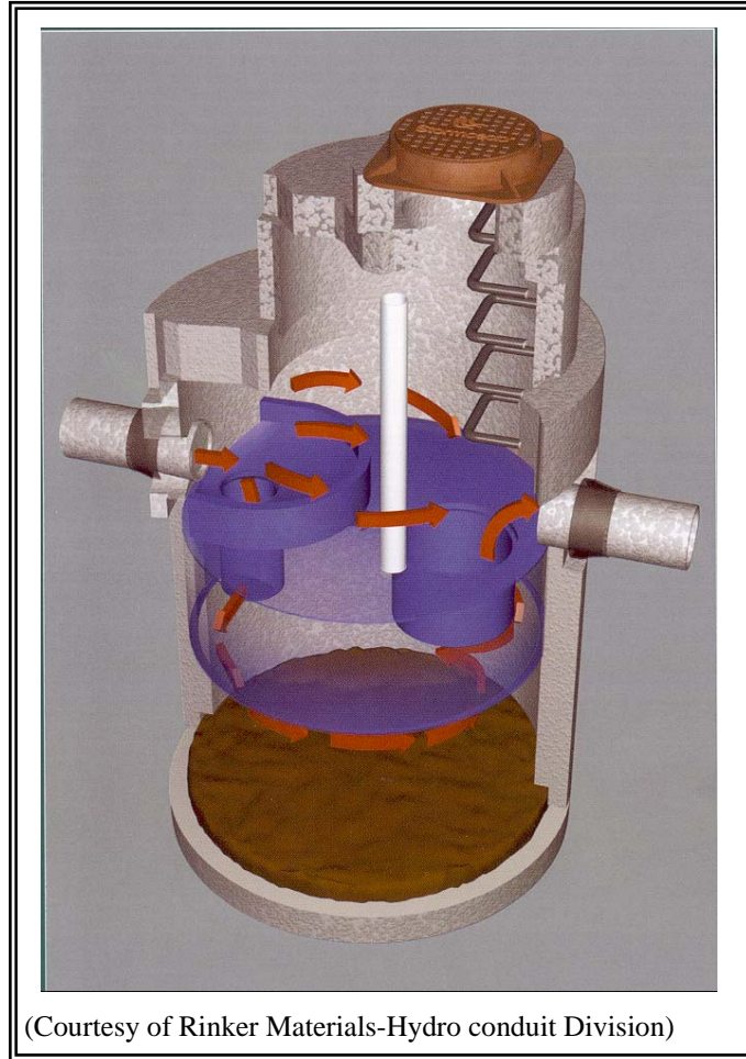
Figure 12.4 – Engineered Cylindrical
