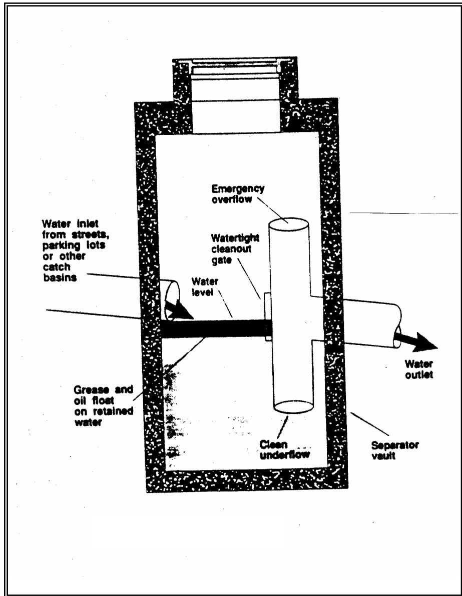
Figure 11.3 – Spill Control Separator (not for oil treatment)
