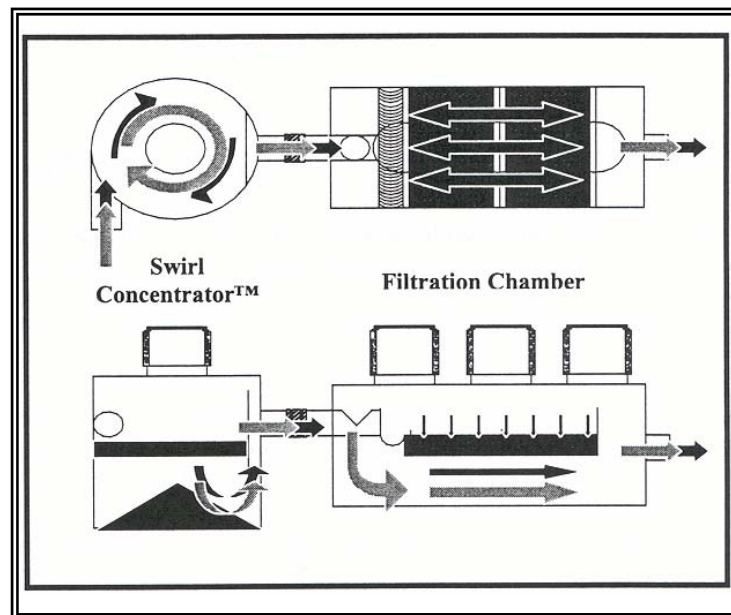
Figure 12.2 - Vortex-enhanced Sedimentation and Media Filtration
