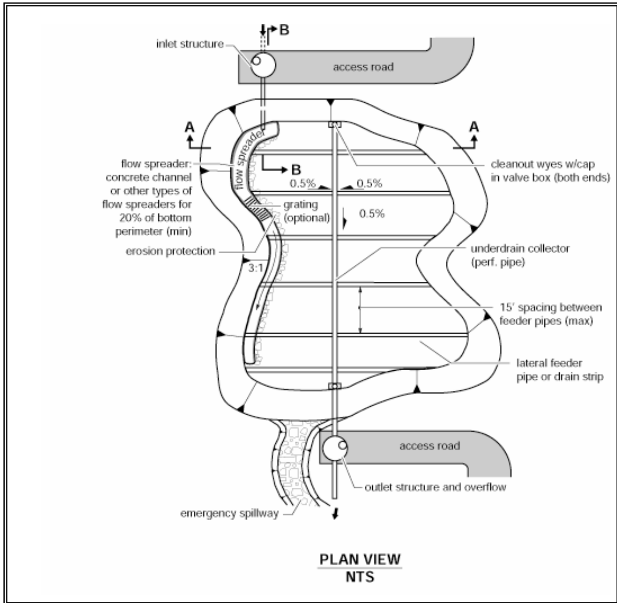
Figure 8.3 – Sand Filter with Level Spreader
