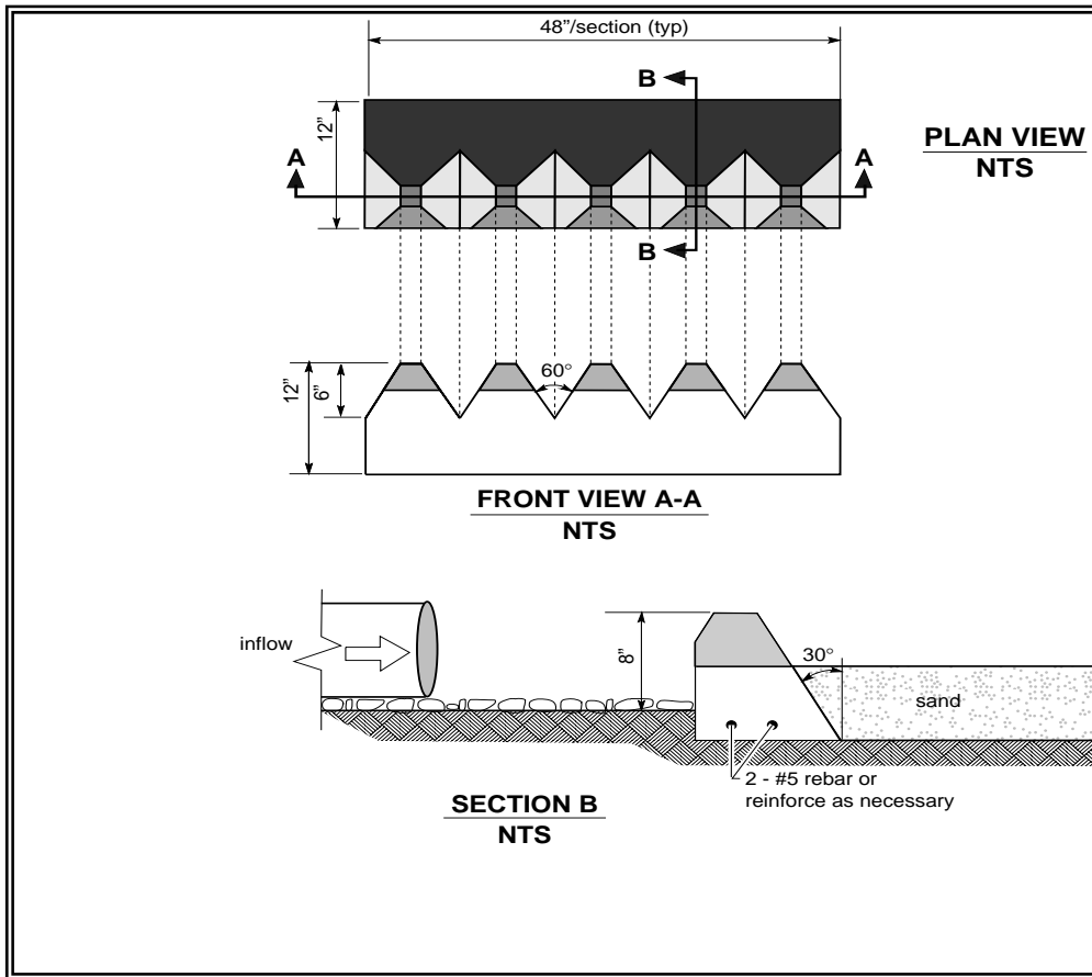
Figure 4.5 – Flow Spreader Option C: Notched Curb Spreader
