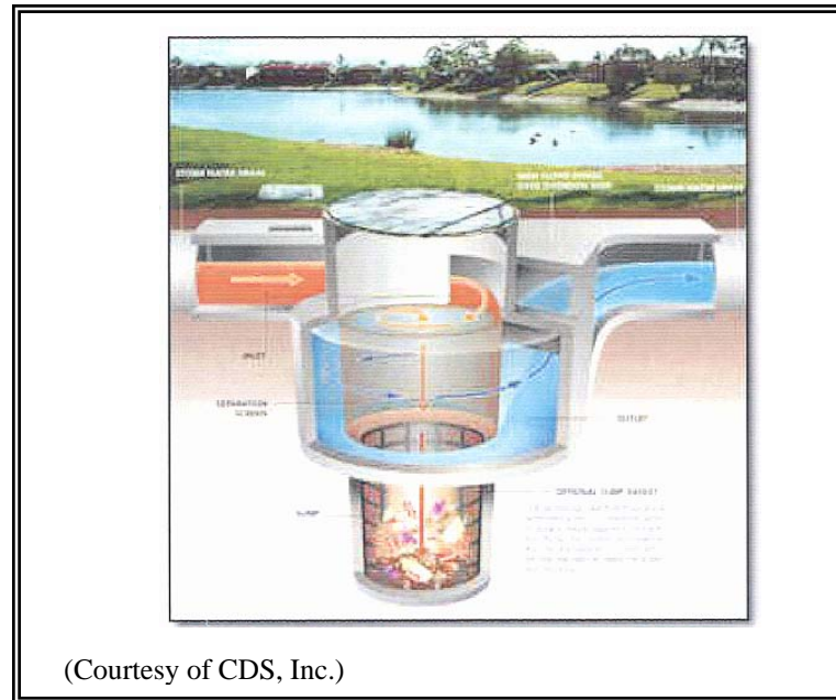
Figure 12.3 – Screen Separator
