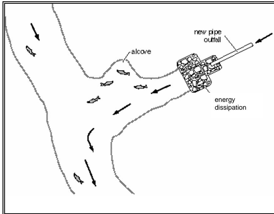
Figure 4.12 – Fish Habitat Improvement at New Outfalls
