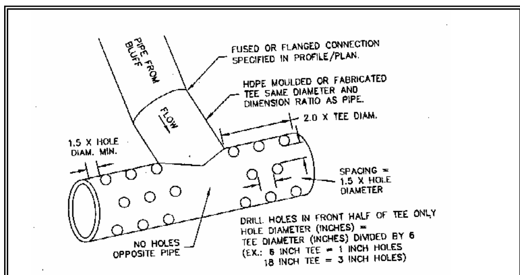
Figure 4.11 – Diffuser TEE (an example of energy dissipating end feature)
