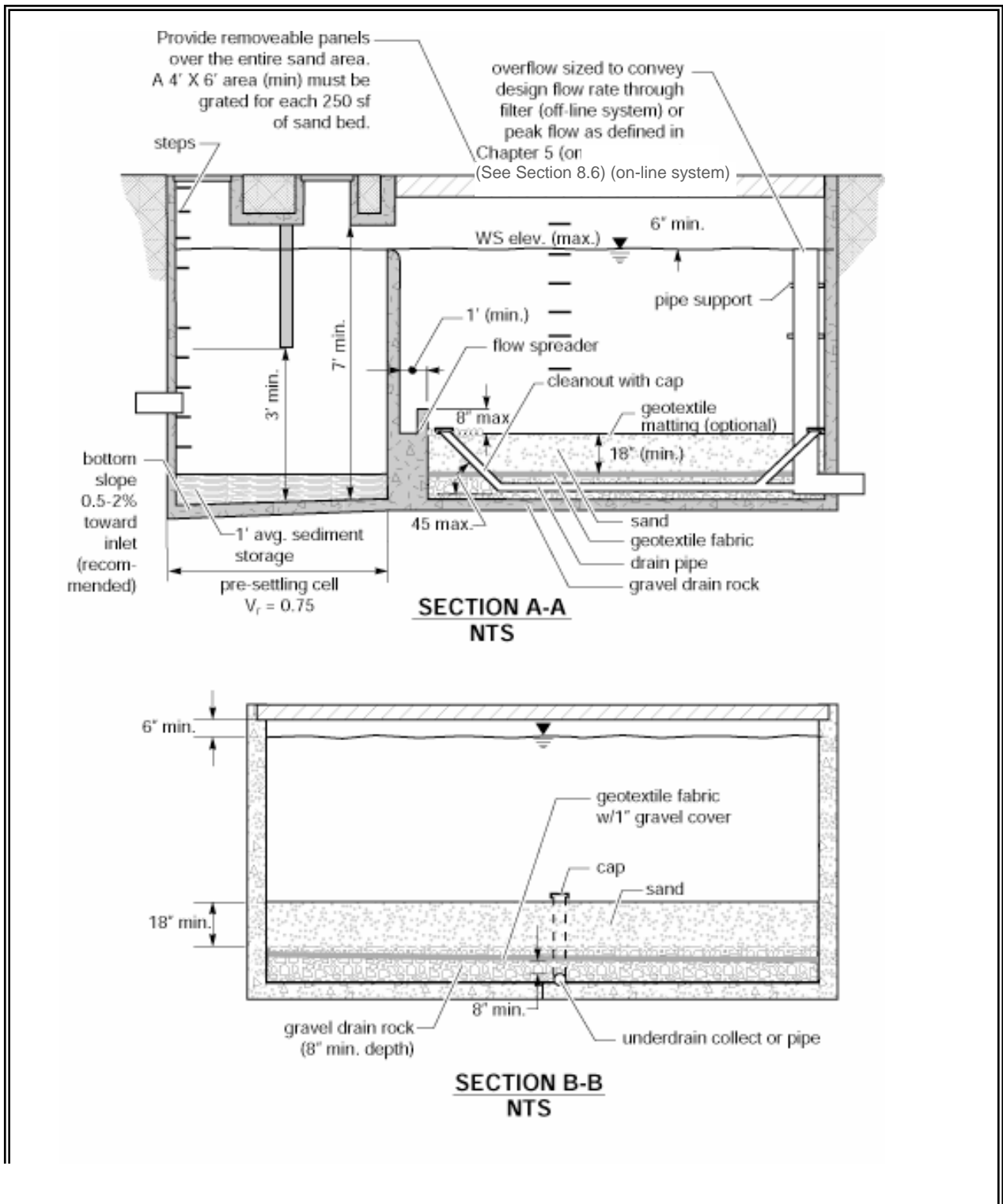
Figure 8.6b – Sand Filter Vault (cont)
