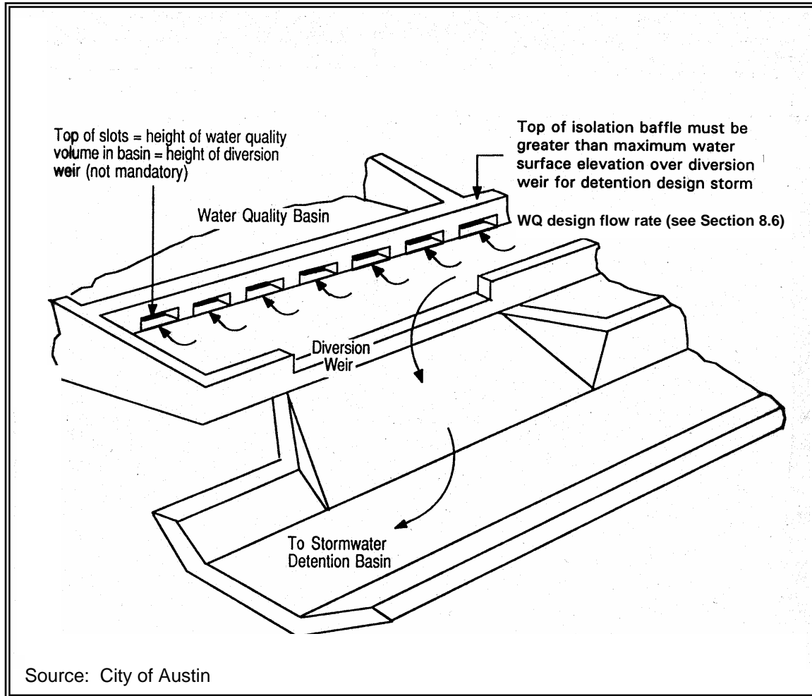
Figure 8.5 – Example Isolation/Diversion Structure
