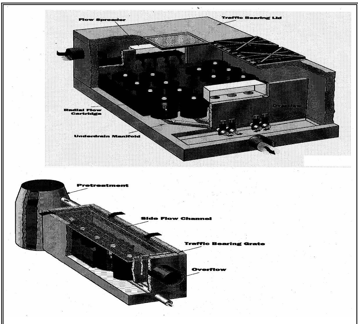
Figure 12.1 – Vertical Media Filter
