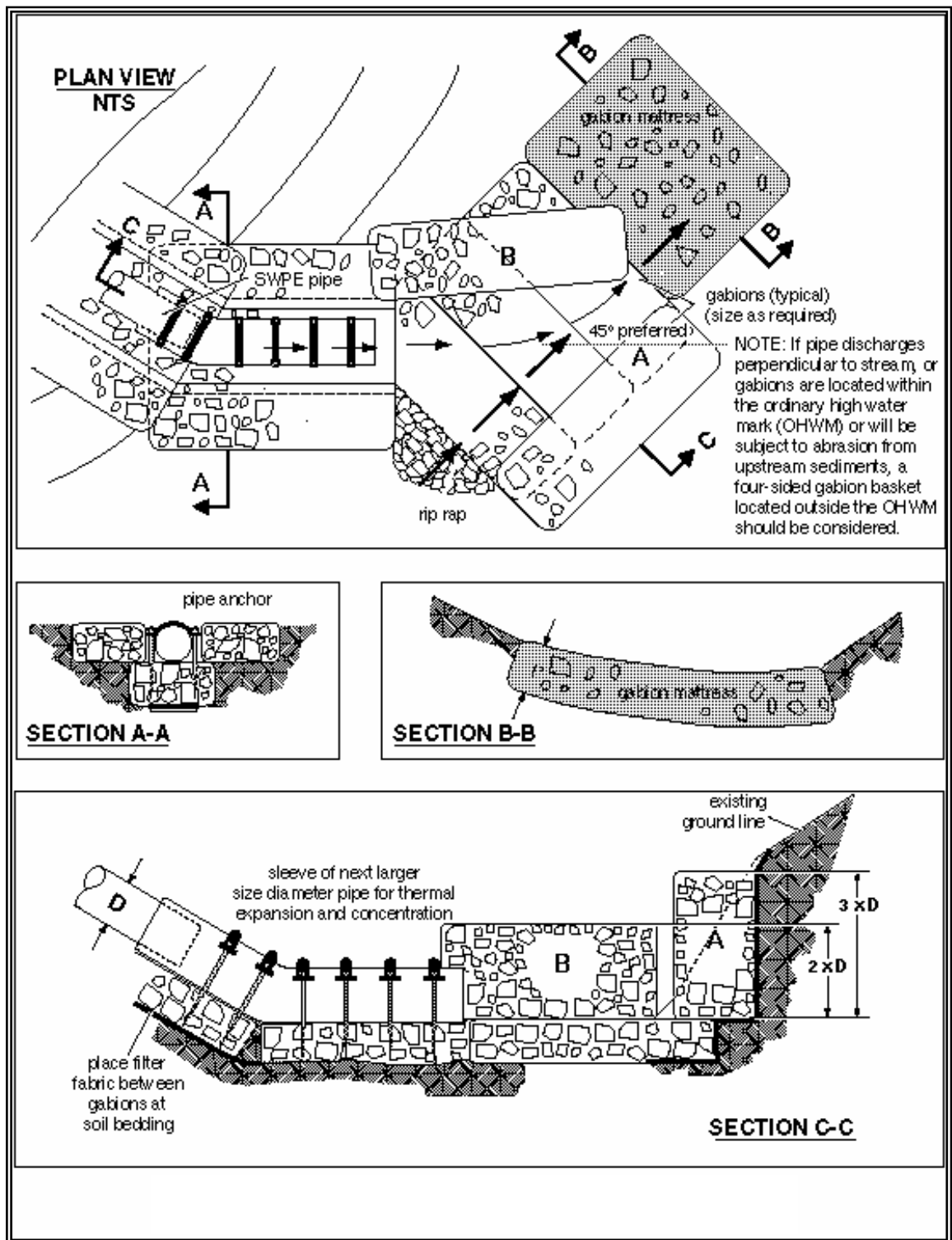
Figure 4.10 – Gabion Outfall Detail
