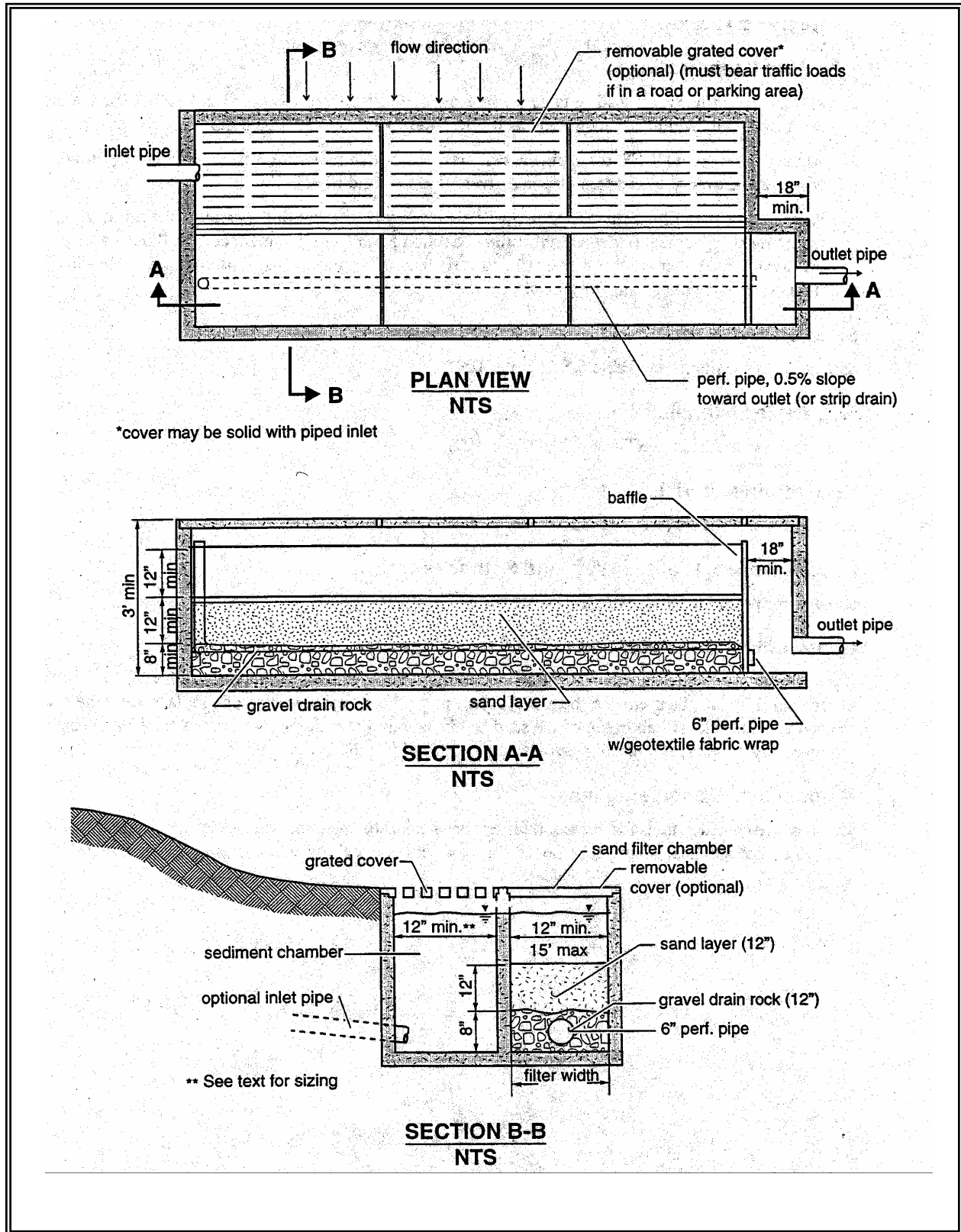
Figure 8.7 – Linear Sand Filter
