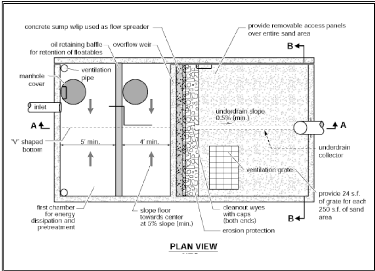
Figure 8.6a – Sand Filter Vault
