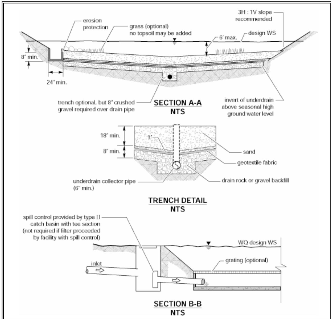
Figure 8.3 (cont) Sand Filter with Level Spreader
