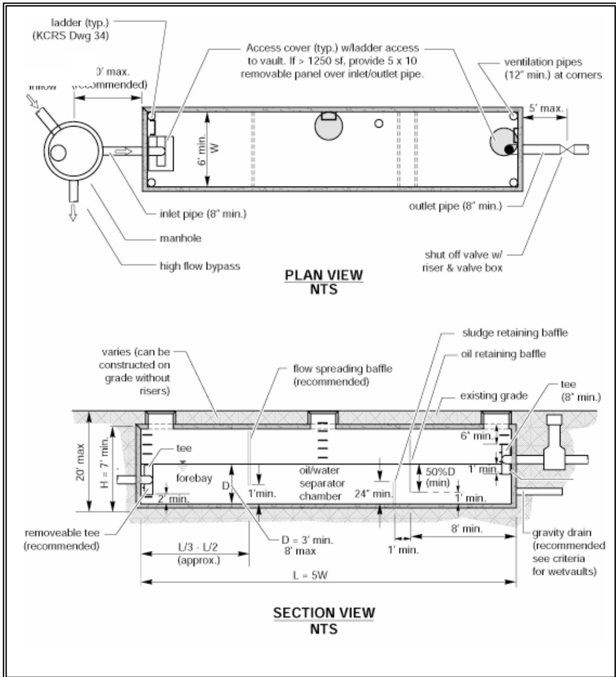
Figure 11.1 – API (Baffle Type) Separator
