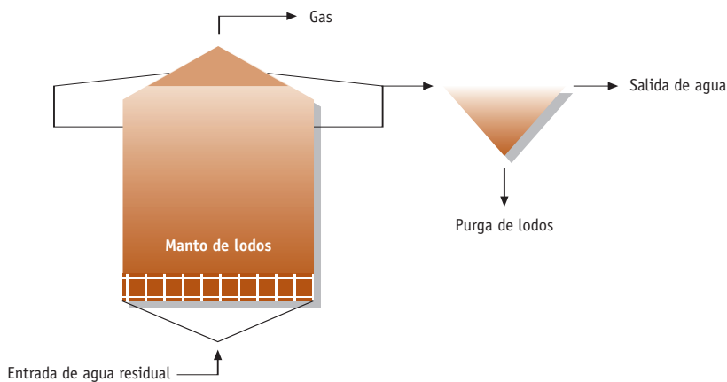
FIGURA 2.6 Reactor UASB.
