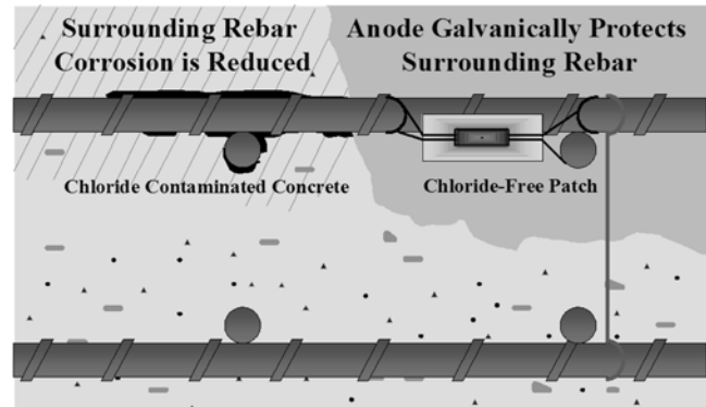
Fig. 2—Chloride-accelerated corrosion.
