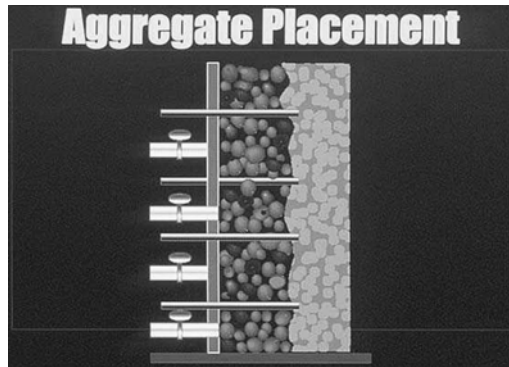
Fig. 3—Aggregate placement
