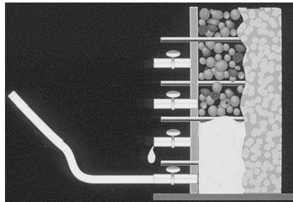
Fig. 4—Pumping grout
