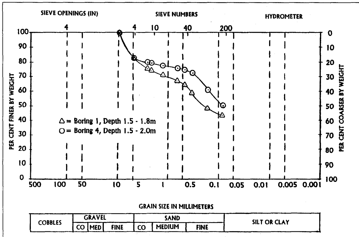
Figure 30. Gradation of landfill deposits, Indiana site.
