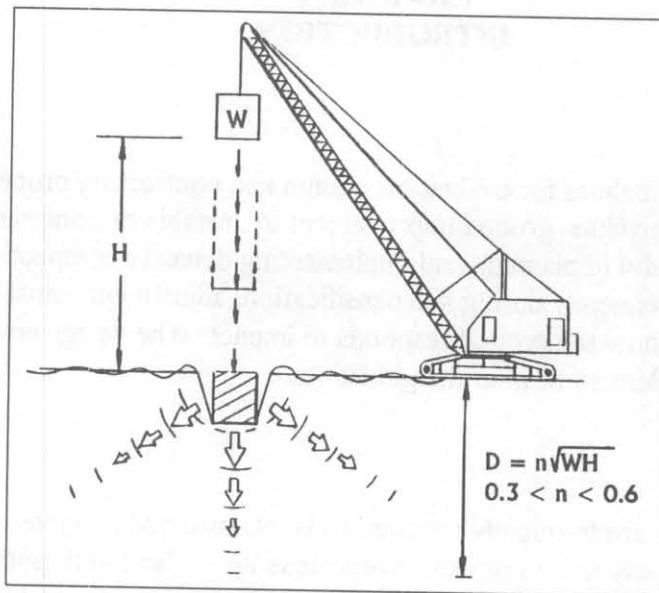
Figure 1. Dynamic compaction.
